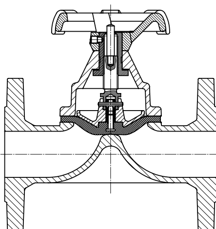
Sectional drawing
