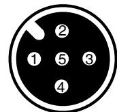
X 3 A-coded M12 socket
