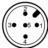
X 1 A-coded M12 plug
