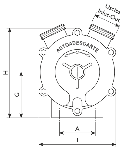
SPECIAL 30-40-50 SPECIAL SENIOR 1"1/2 SPECIAL MASTER 2"
