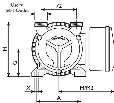
EPH NEOS 3/4" EP NEOS 3/4"
